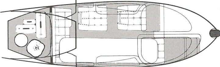
AIR AMBULANCE Stretcher fits through nose door Pilot and attendant have left side entry door
