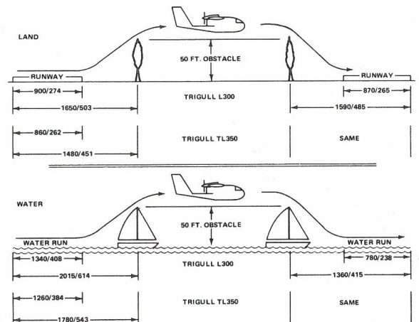
TAKE-OFF AND LANDING DISTANCES (FEET/METERS), SEA LEVEL, STANDARD DAY, GROSS WEIGHT
